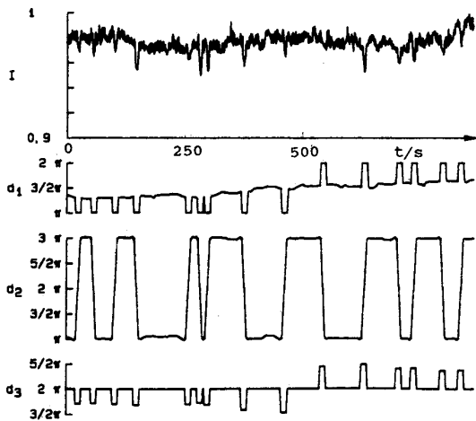
Fig. 5. d_2 resets from different d_1 starting points.
