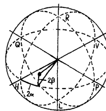
Fig. 1. Poincaré sphere.
