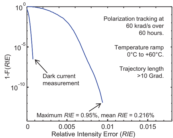
Fig. 3. Complementary cumulative distribution function 1-F(\text{RIE}) of relative intensity error at 60 krad/s input polarization scrambling and 60 °C temperature changes over 60 h.
