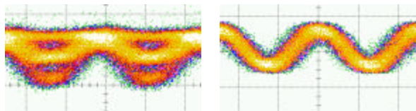
Fig. 2: Back-to-back 40 Gbaud intensity “eye” diagrams of NRZ-DQPSK (left) and RZ-DQPSK signals (right).
