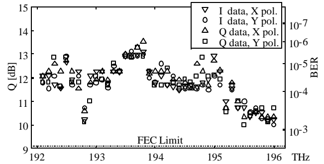
Fig. 6: Measured BERs and corresponding Q factors, in phase and in quadrature in both polarizations for all 40 channels after 324 km of fiber, as a function of optical frequency.
