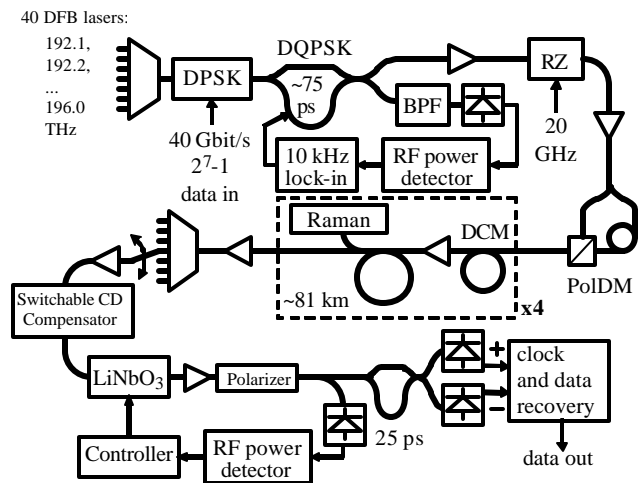
Fig. 1: 40 \times 2 \times 2 \times 40 Gbit/s RZ-DQPSK polarization division multiplex transmission setup.
