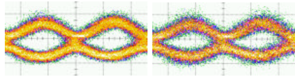
Fig. 7: Interferometrically demodulated eye diagrams at 40 Gbit/s before (left) and after transmission (right) in 193.8 THz channel in one polarization and one quadrature.
