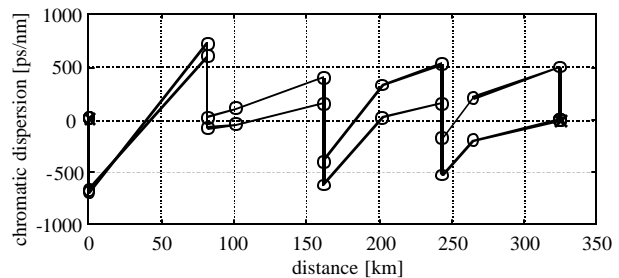
Fig. 3. Accumulated chromatic dispersion at 1530 and 1561 nm vs. distance. Connectors are marked by circles, transmit and receive ends by circled x.
