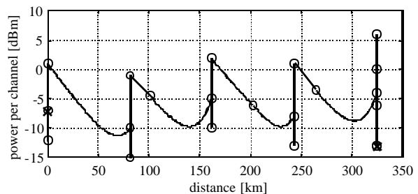
Fig. 4. Power of a typical 160 Gbit/s WDM channel vs. distance. Connectors are marked by circles, transmit and receive ends by circled x.
