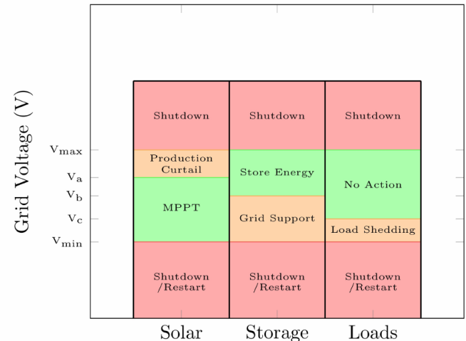
Grid Voltage Protocol for the PeCo Grid
